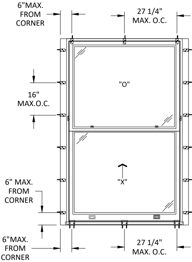
ANCHOR LAYOUT HRS12 STRAP BENT AROUND FRAME INSTALLATION
