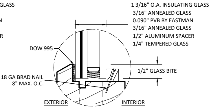
GLAZING DETAIL 2
