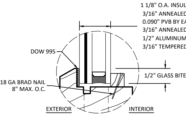
GLAZING DETAIL 1
